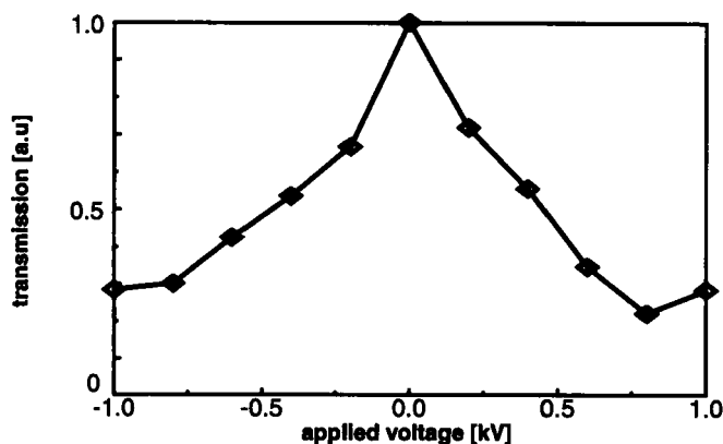
FIGURE 5. Transmission of the waveguide in dependence of the applied voltage. The spectral hole was burned and poked at 634 nm with the diode laser.
