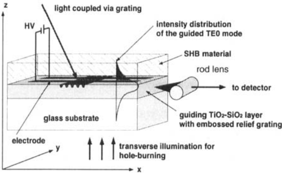
FIGURE 1. Construction of the waveguide.
