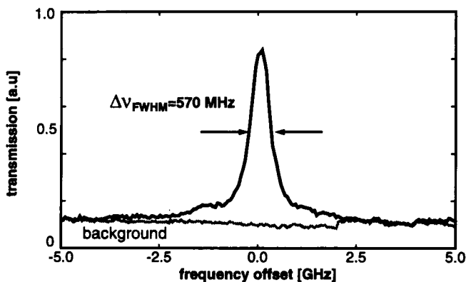
FIGURE 4. Waveguide spectral transmission after transverse illumination with 110-MHz-line-width diode laser (black line). Gray line - background signal level (mostly scattered light) measured before hole-burning.
